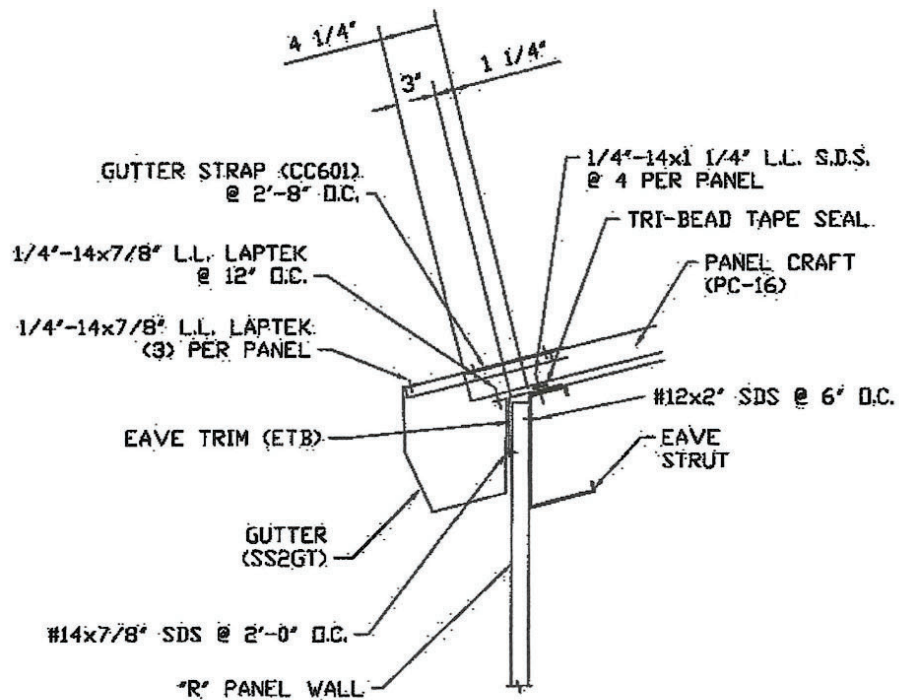
GUTTER DETAIL
